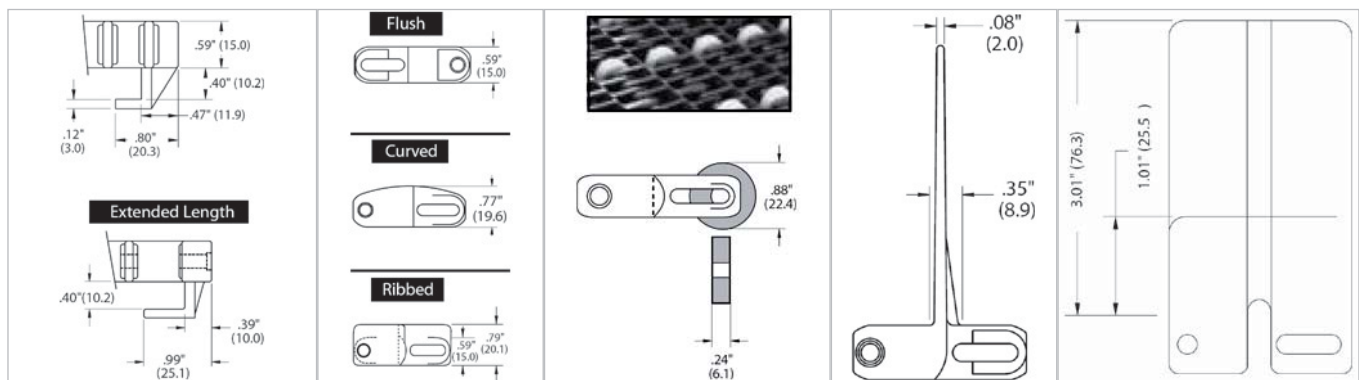
Hold-down tabs
