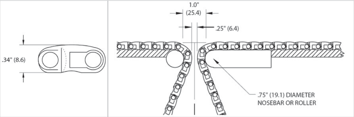
Inserts Note: Inserts may affect belt pull
