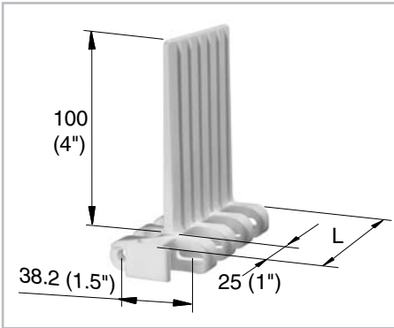
Edge flight M384RF10 (right side) M384LF10 (left side) The total length L of the right and left type add to 200 mm (8")
