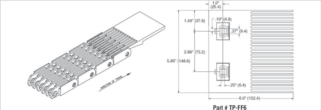
Fluid-Flo transfer plate
