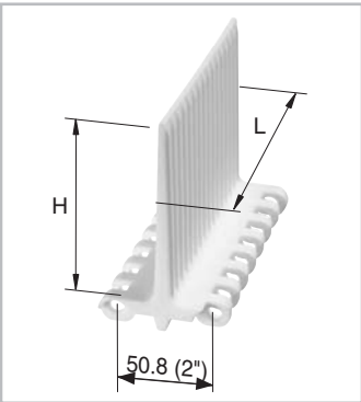
M5010Fxx "no-cling" side
