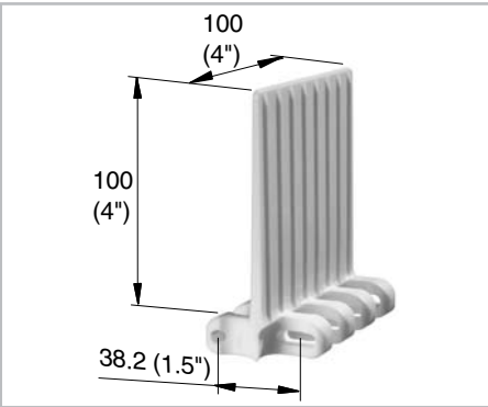
Middle flight M3840F10
