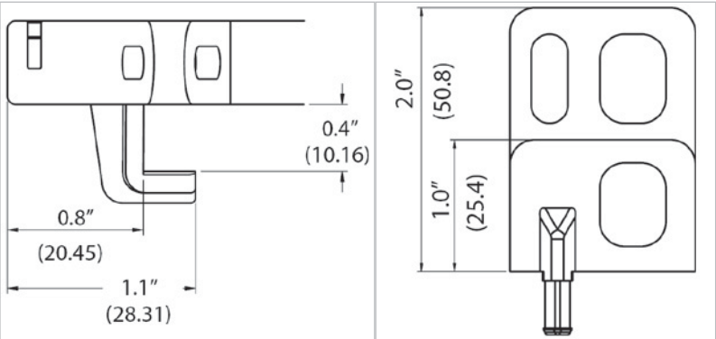
Hold-down tabs
