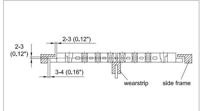
Side tabs M2544
