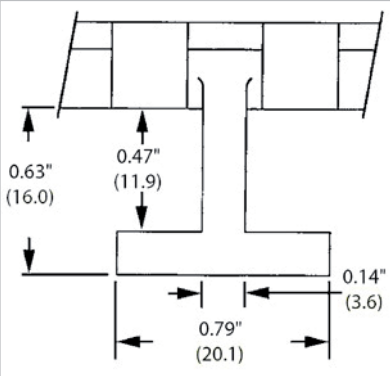
Hold-down tabs
