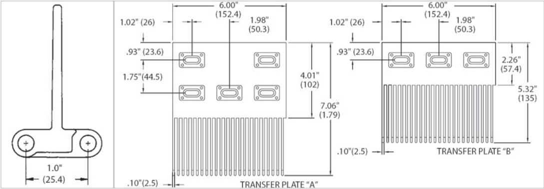
Flights Standard flights are available in 1" and 2" heights
